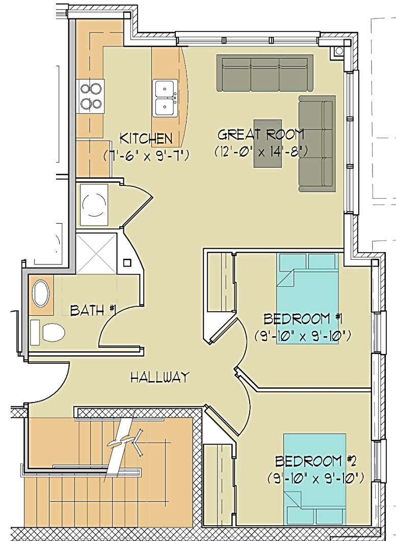
LOWER LEVEL
